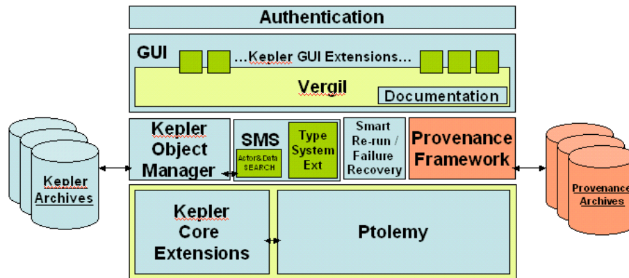
Fig. 1. The Kepler System Architecture
