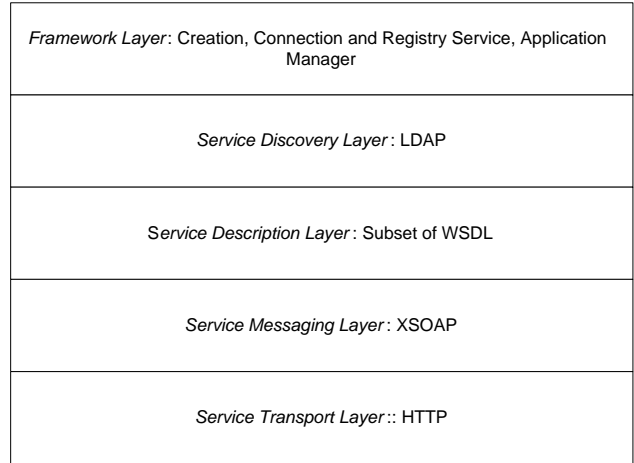
Figure 3. Each layer of the Web Services stack has a corresponding layer in each XCAT component.
