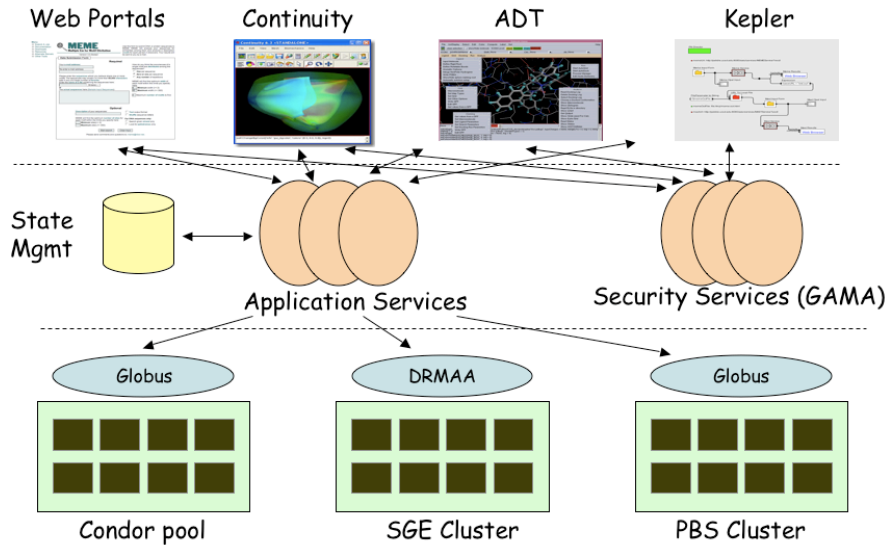
Fig. 1. NBCR SOA Architecture
