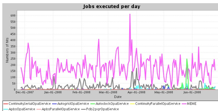
Fig. 4. Job statistics via the Opal dashboard
