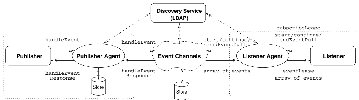
Figure 10: The Event Subsystem
